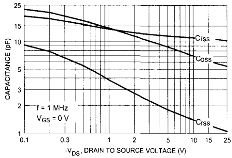
Figure 8. Capacitance Characteristics.
