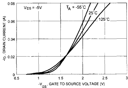
Figure 5. Transfer Characteristics.
